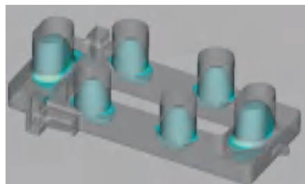
凝固模拟 Solidification simulation
